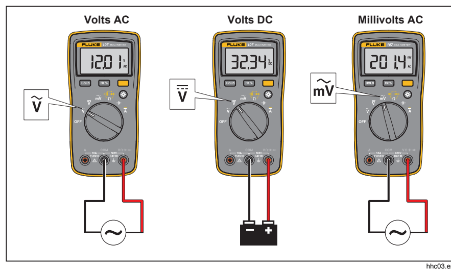
Figure 2. Measure AC and DC Voltage
